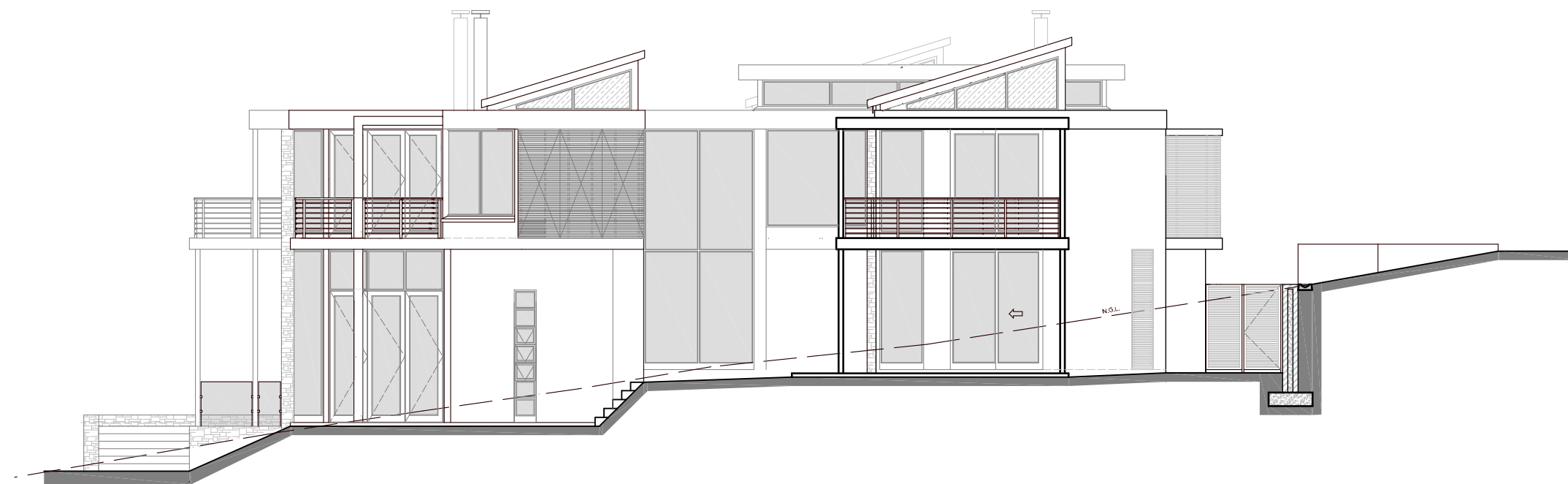
WESTERN ELEVATION
